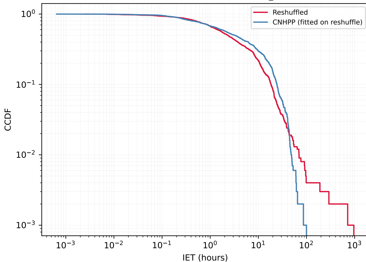
User 274636082 - Reshuffled vs CNHPP A_{\text{fit}}=0.2152
